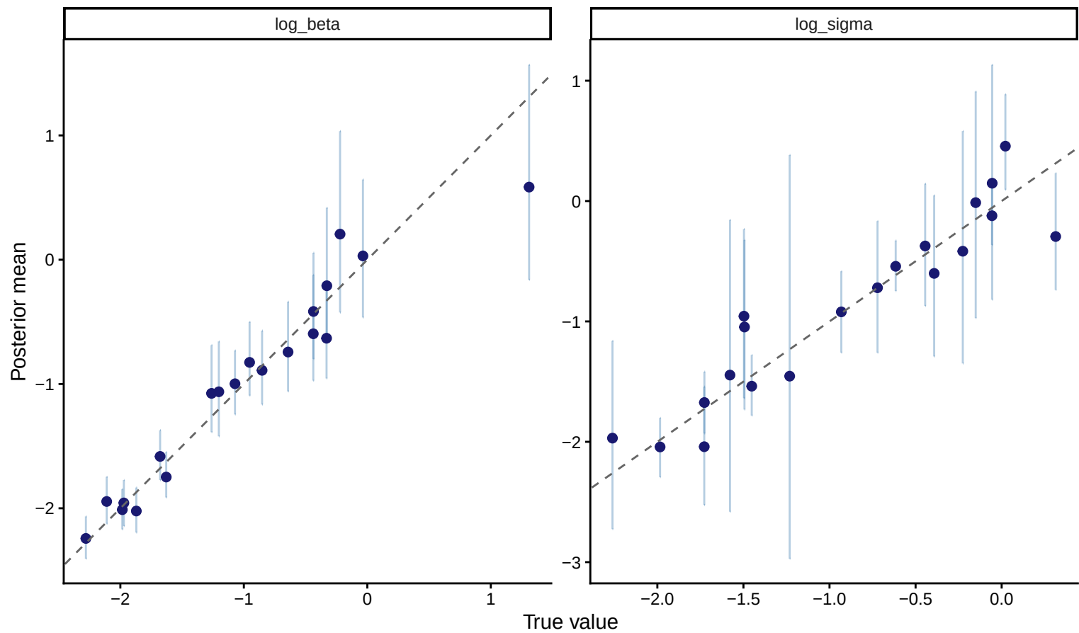
0-ToM parameter recovery (20 agents, 200 trials)
