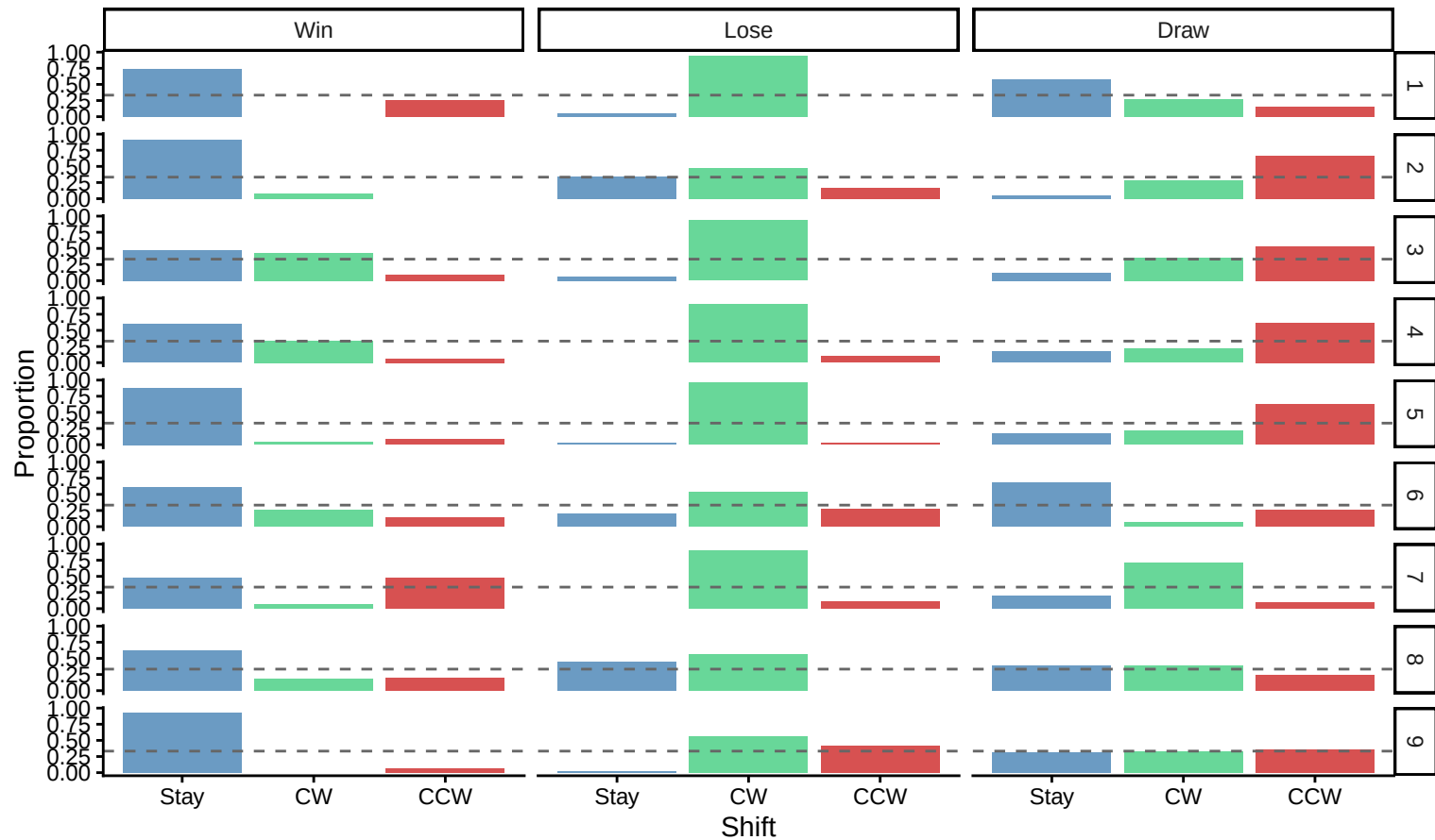
WSLS prior predictive: 9 prior draws \times 3 outcomes
