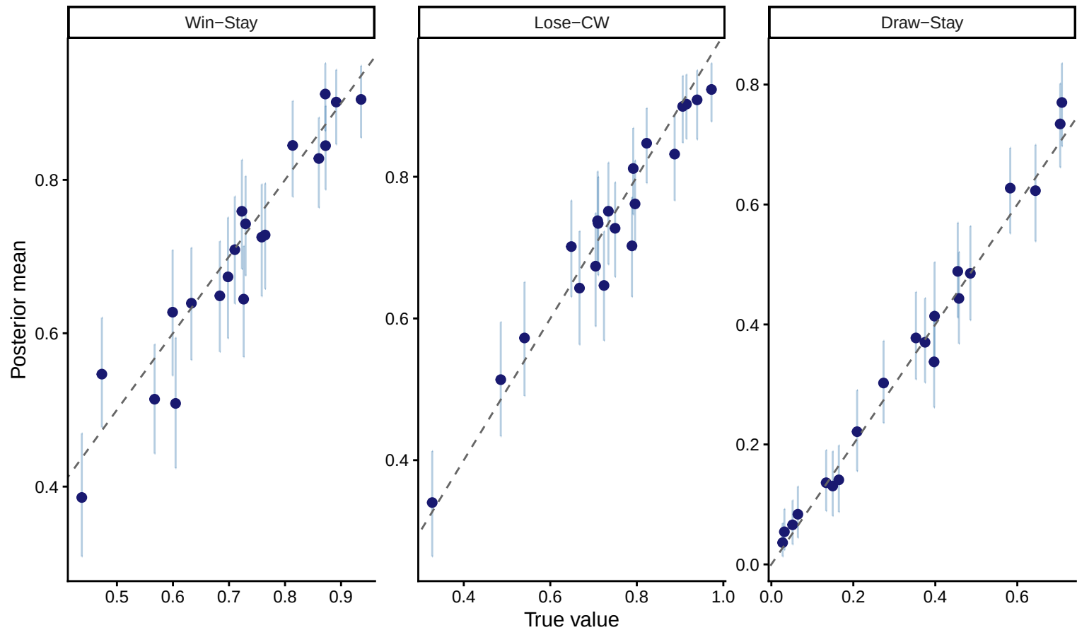
WSLS parameter recovery (20 agents, 300 trials)
