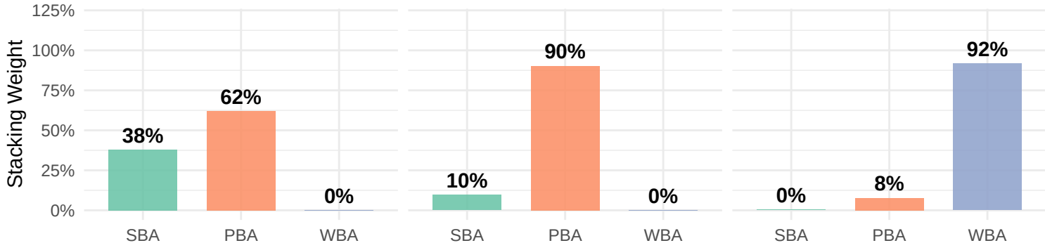
Multilevel Stacking Weights
