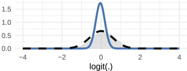
Population Distribution: logit(.)
