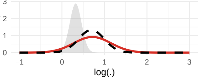
Population Distribution: log(.)
