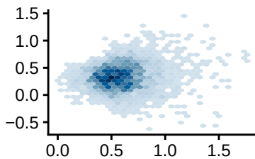
pop_log_r_sd
