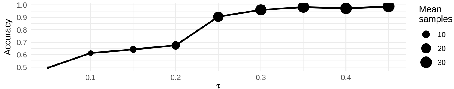
(b) Accuracy vs. threshold
