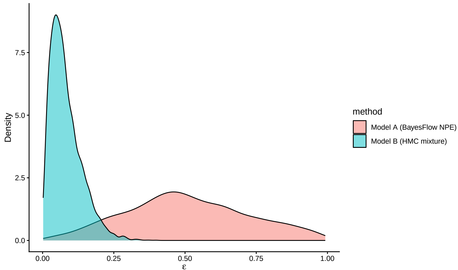
Model A vs Model B posterior on epsilon
