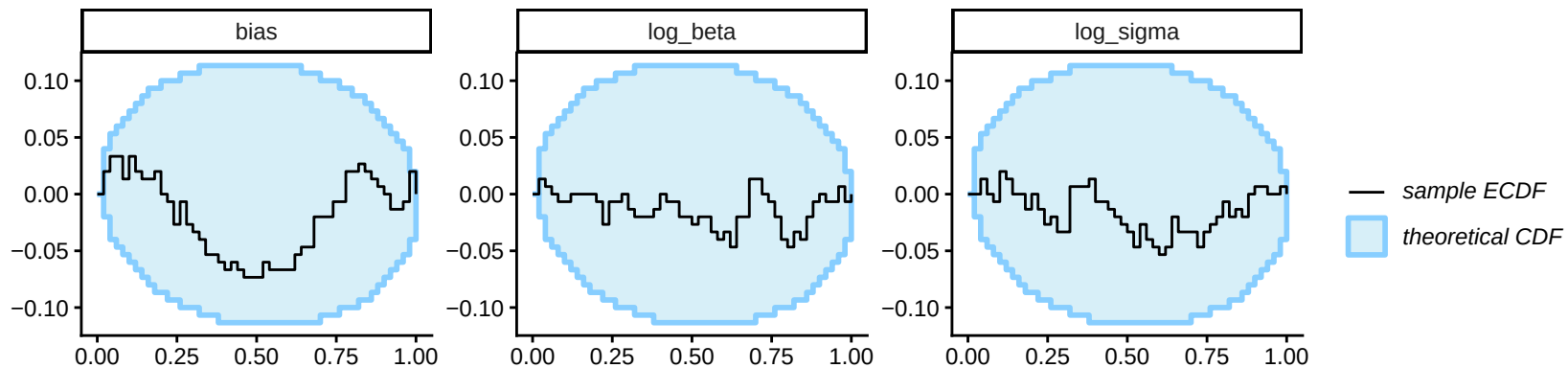
ECDF difference
