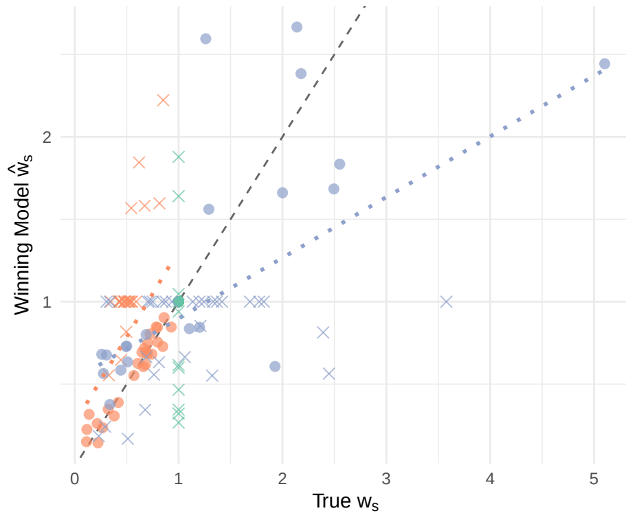
Recovery of w_s
