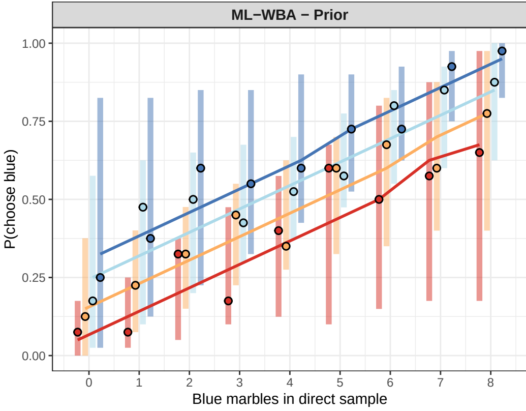
ML-WBA Prior Population Prior Predictive Check
