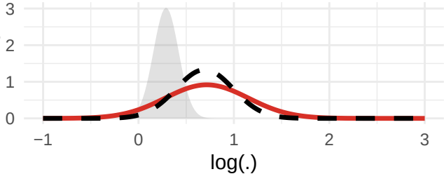
Population Distribution: log(.)
