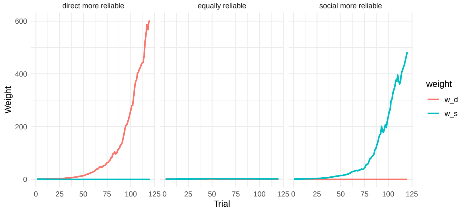
(a) Weight trajectories by regime
