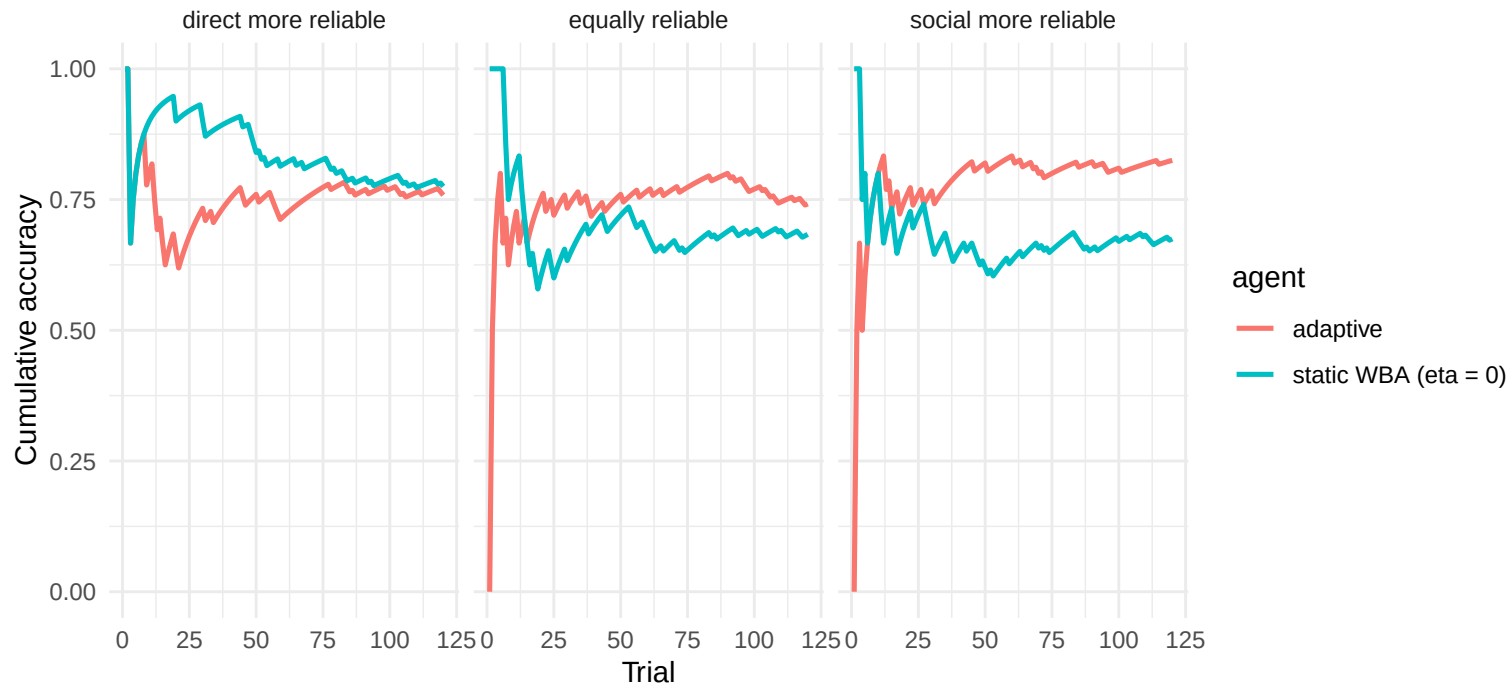
(b) Running accuracy: adaptive vs. static WBA
