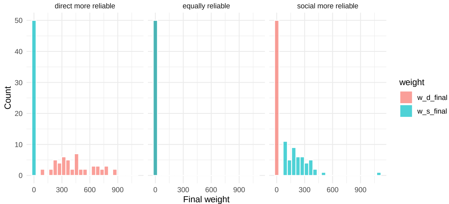
(c) Final-weight distribution (50 agents per regime)
