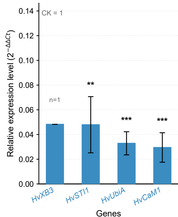
A Barley candidate genes
