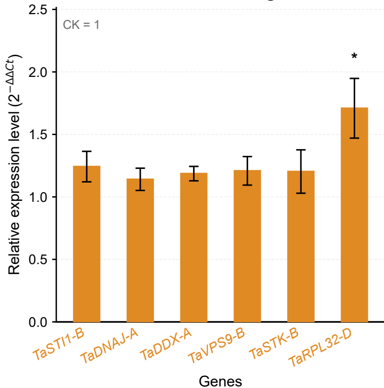
B Wheat candidate genes
