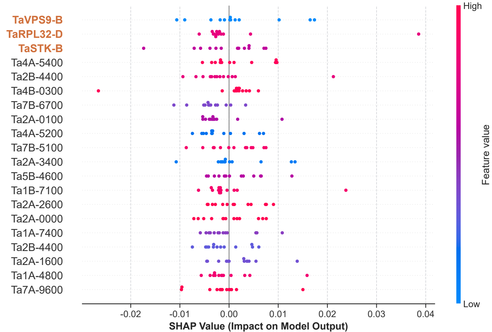
Wheat: SHAP Global Importance
