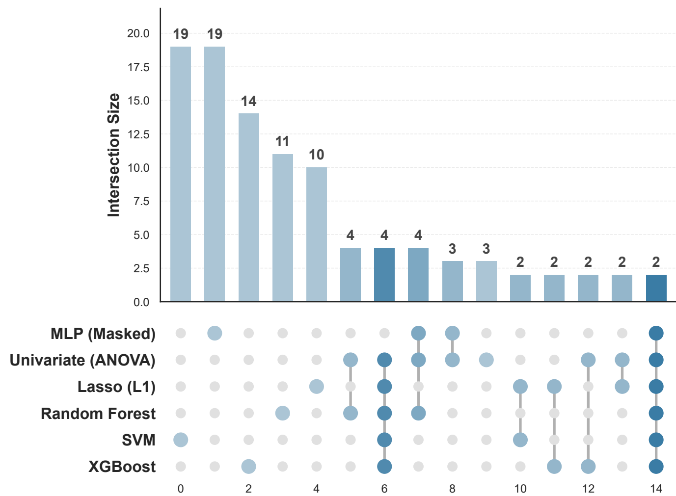
Barley: Models Consensus (UpSet)
