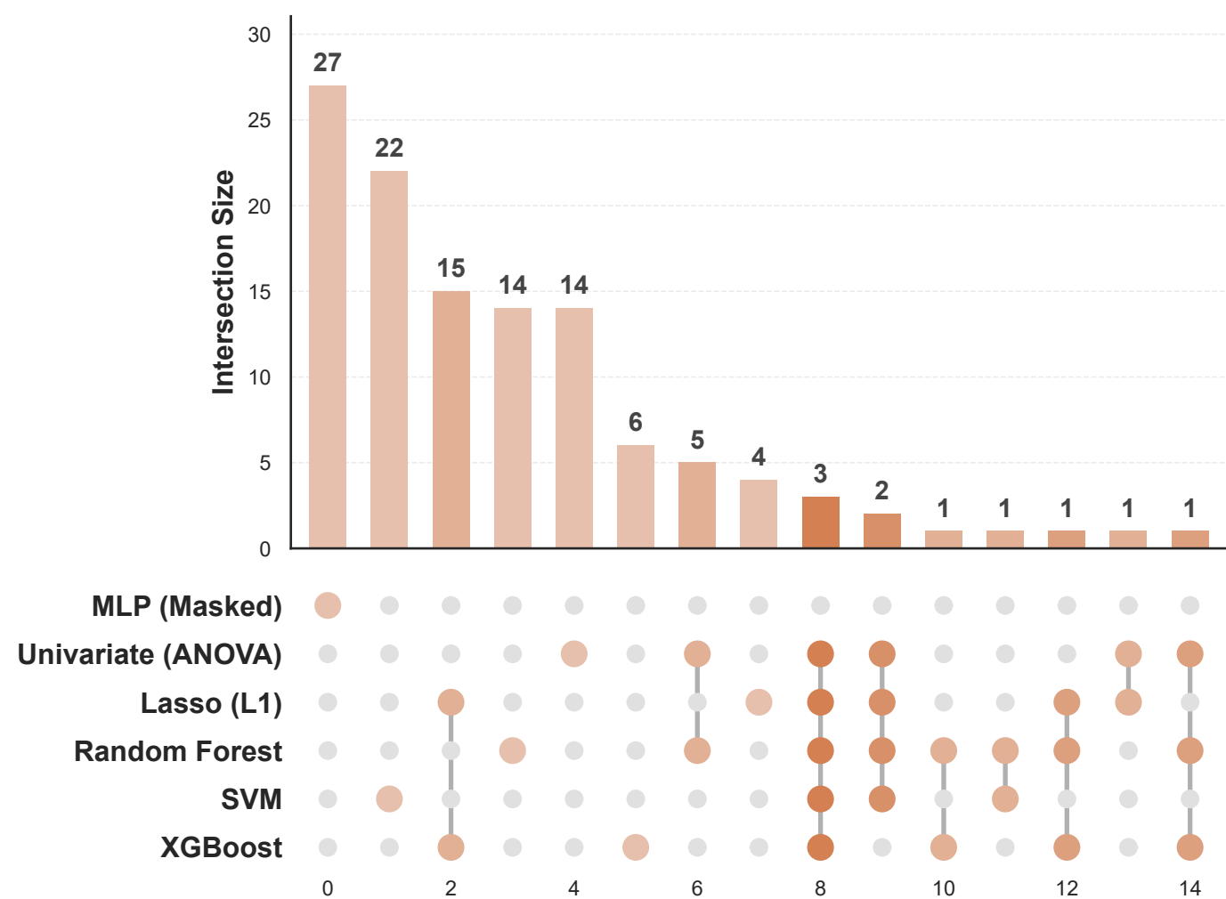
Wheat: Models Consensus (UpSet)
