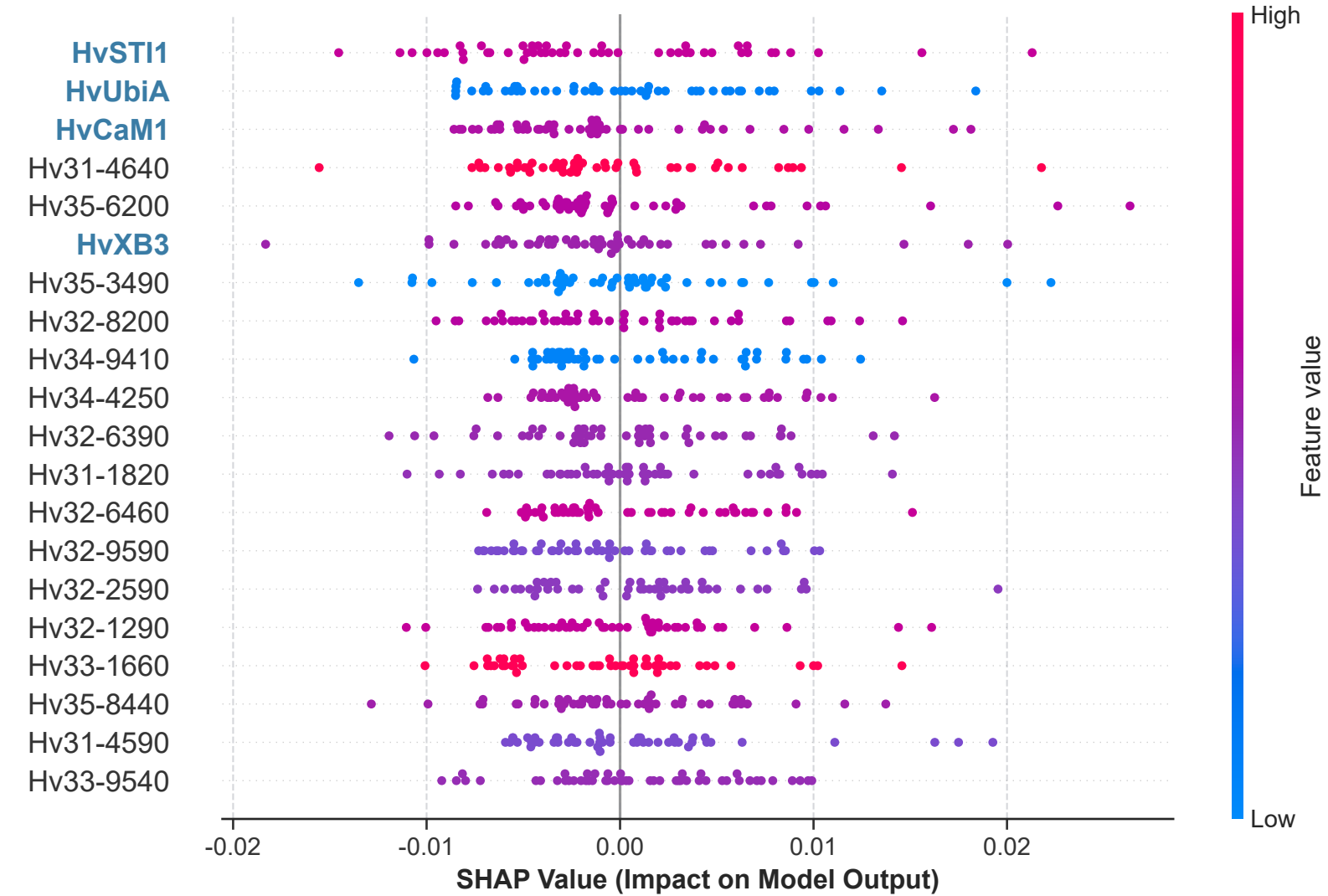
Barley: SHAP Global Importance
