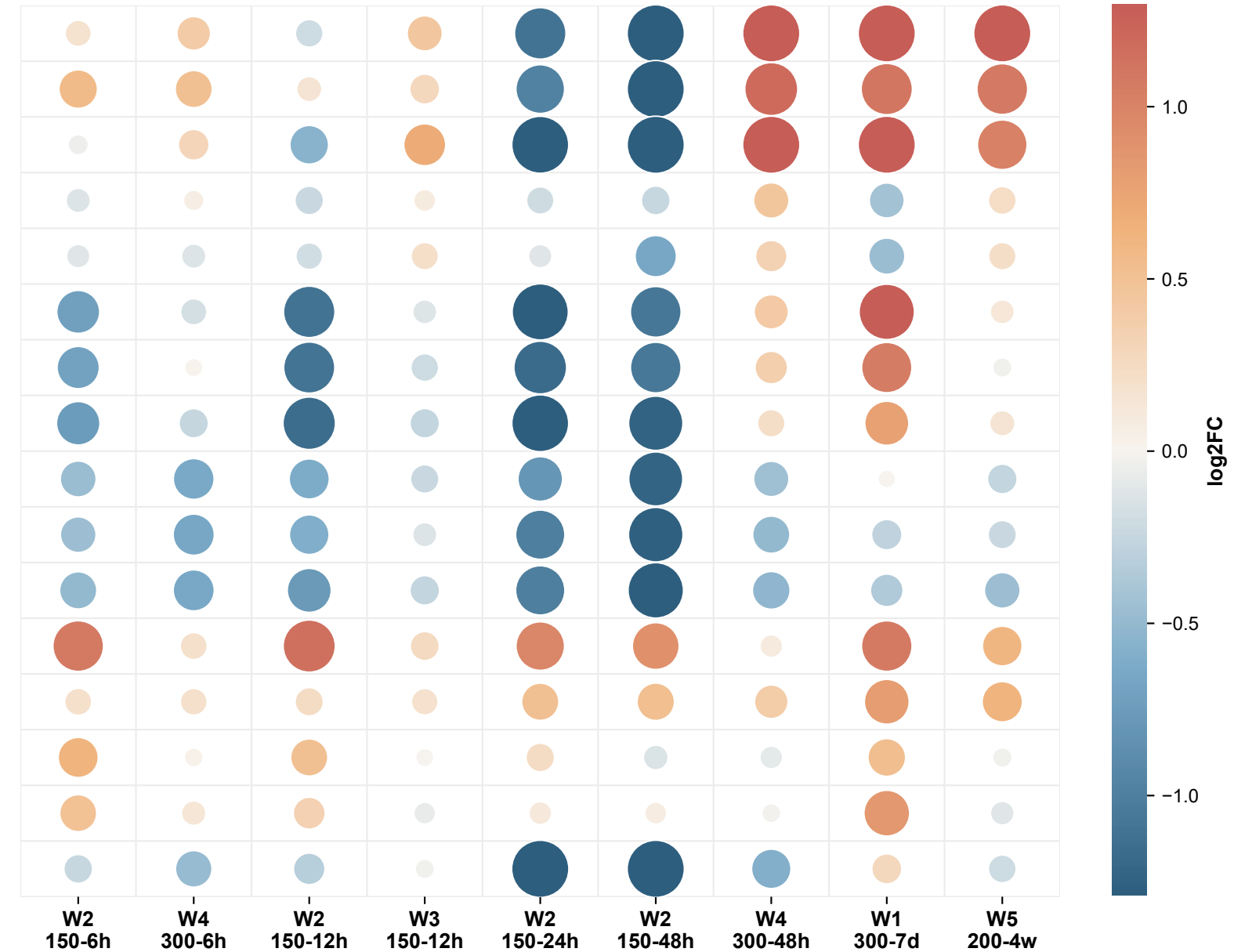
Wheat log2FC vs paired CK
