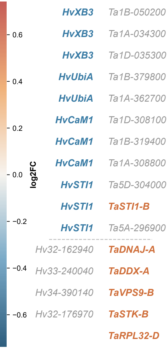
Orthologous Gene Pairs
