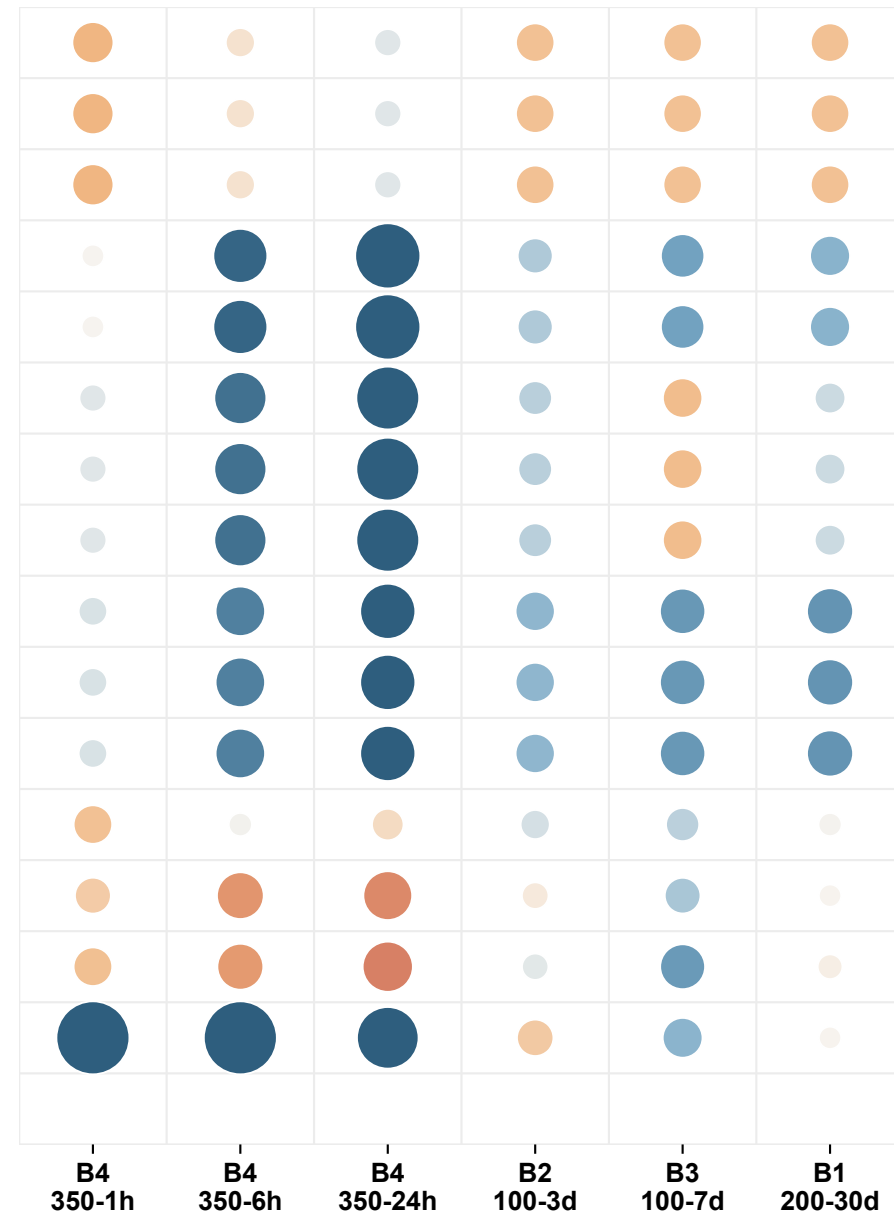
Barley log2FC vs paired CK
