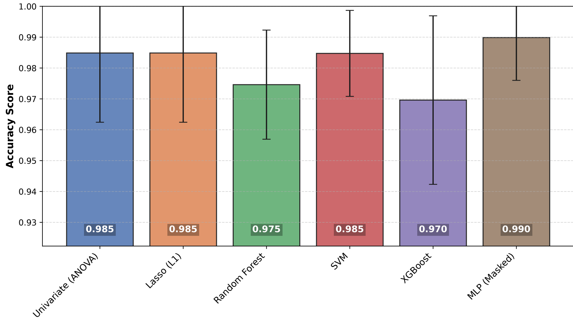
Mean Performance by Algorithm (5-Fold CV)
