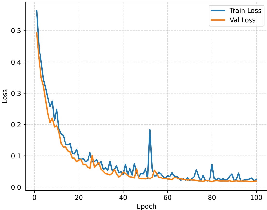
MLP Learning Curve
