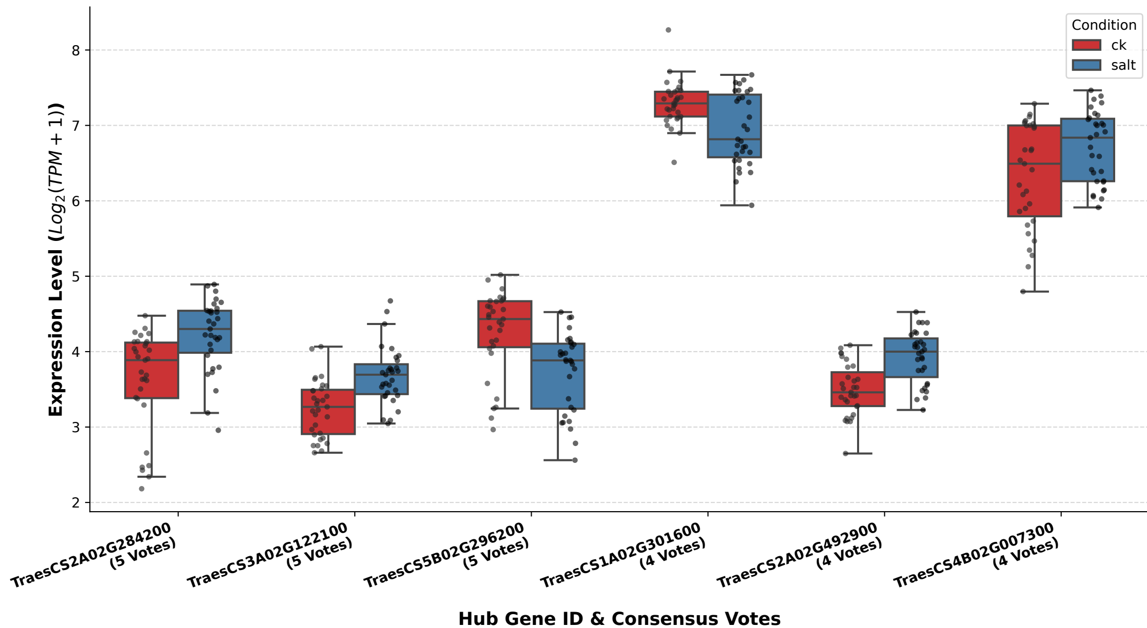
Fig I: Validation of Hub Genes Expression (Ranked by Model Consensus Votes)
