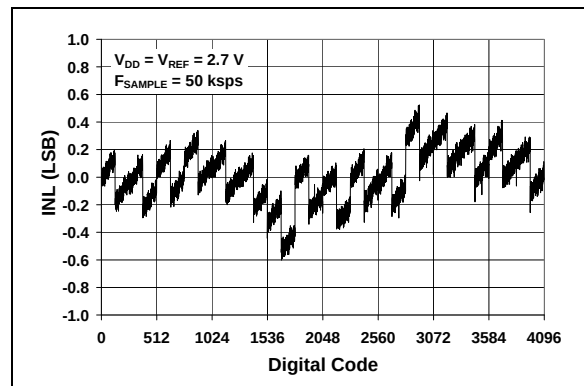
FIGURE 2-6: Integral Nonlinearity (INL) vs. Code (Representative Part, V_{DD} = V_{REF} = 2.7V ).
