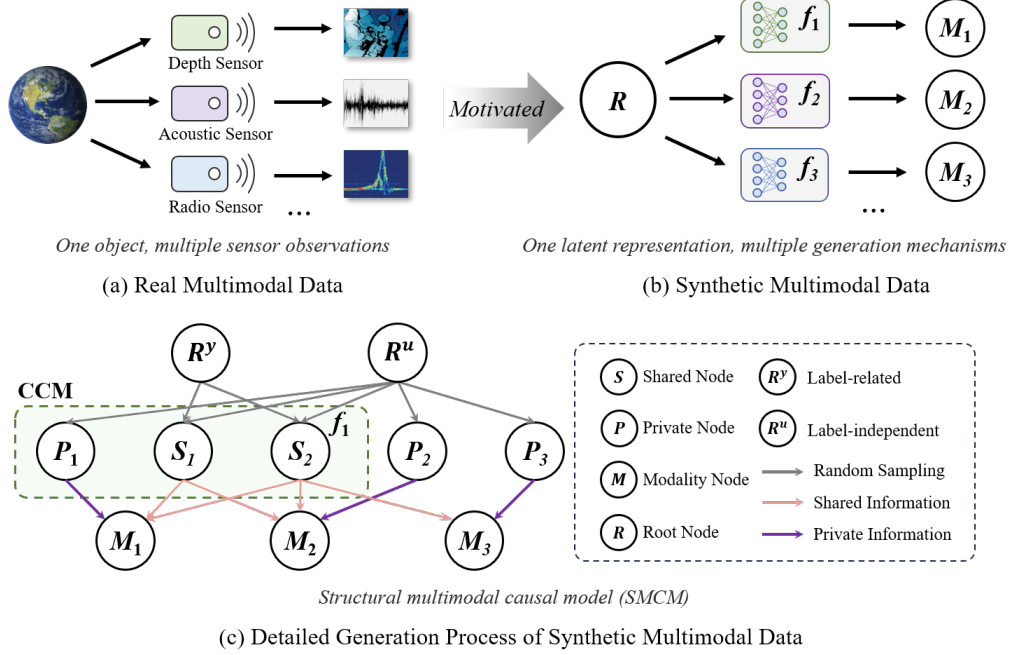
Figure 2: Synthetic multimodal dataset generation process. (a) Real-world multimodal observations are produced by different sensors perceiving the same underlying object or state. (b) Motivated by this process, synthetic modalities are generated from a common latent representation through distinct generation mechanisms in this paper. (c) An example SMCM with three modalities M_1 , M_2 , and M_3 , where the root representation is decomposed into label-related and label-independent components, and the CCM organizes their allocation across shared and private nodes. Shared nodes connect to multiple modality nodes to introduce common information to different modalities, whereas each private node is associated exclusively with its corresponding modality to preserve modality-specific variation. Through different configurations of shared and private nodes, the SMCM induces diverse correlations among M_1 , M_2 , and M_3 .
