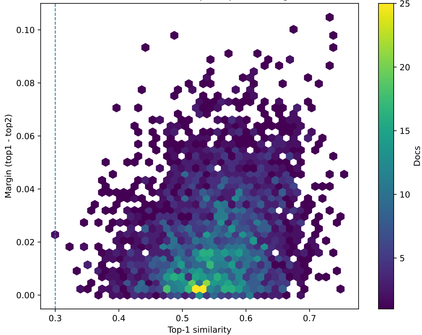
Confidence landscape: top-1 vs margin
