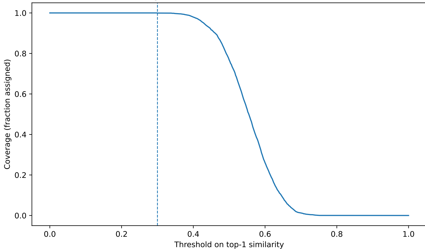
Coverage vs threshold (from score distribution)
