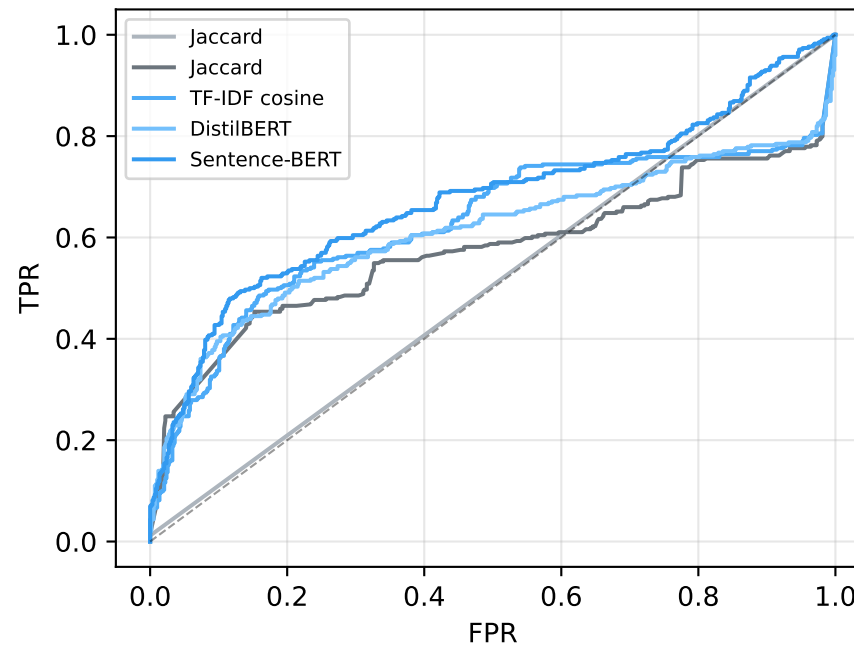
ROC (full eval set)
