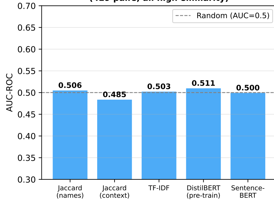
AUC on Pre-filtered Pairs (429 pairs, all high-similarity)
