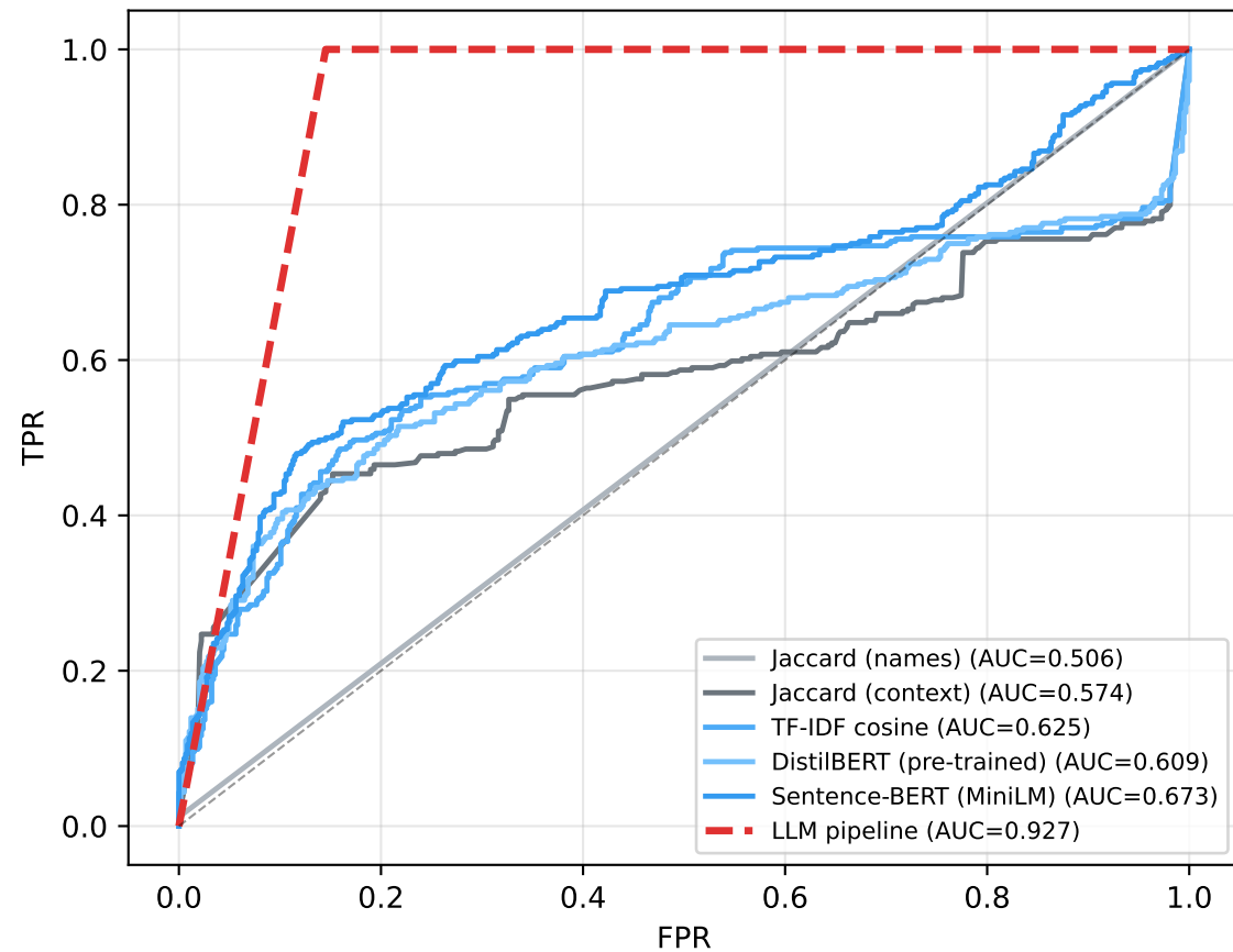
ROC Curve
