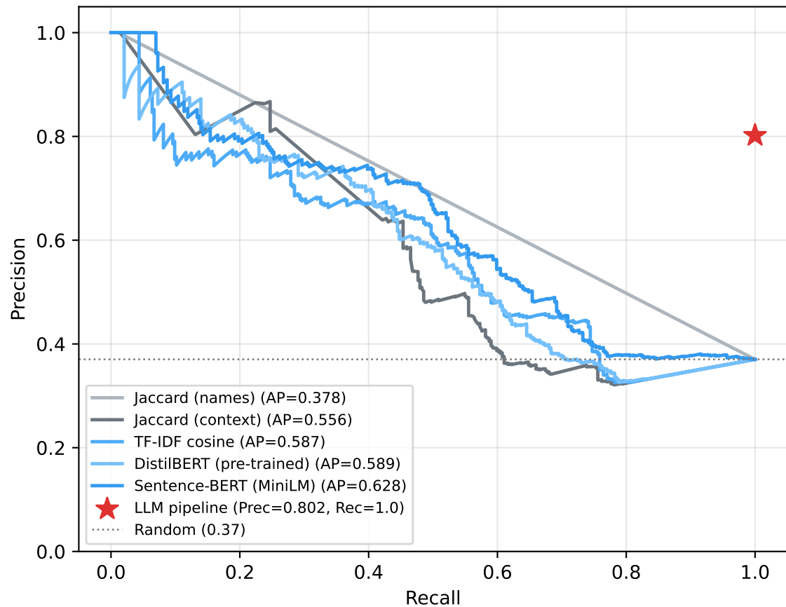
Precision-Recall Curve
