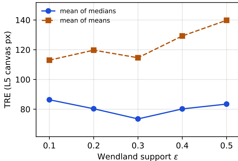
SuperPoint + LightGlue
