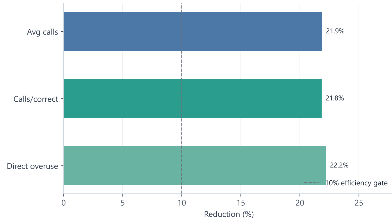
Efficient GRPO effect
