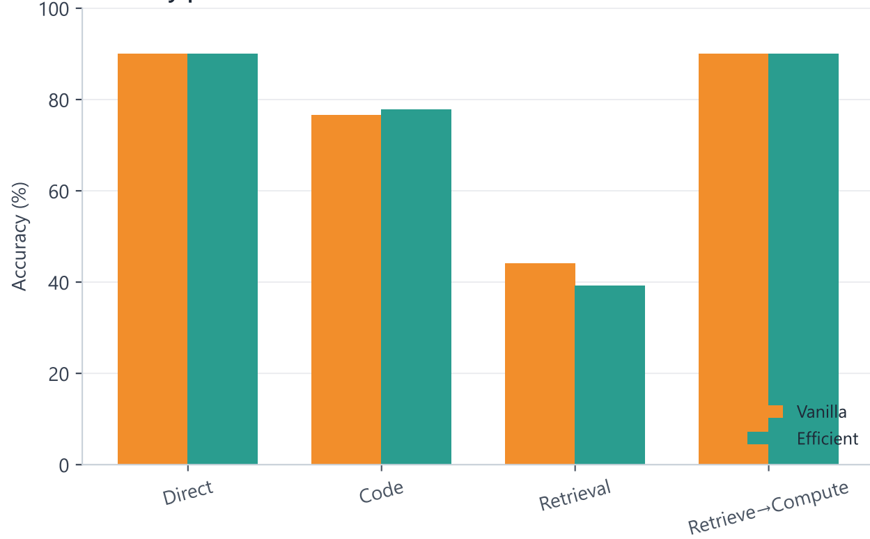
Accuracy preserved across task families
