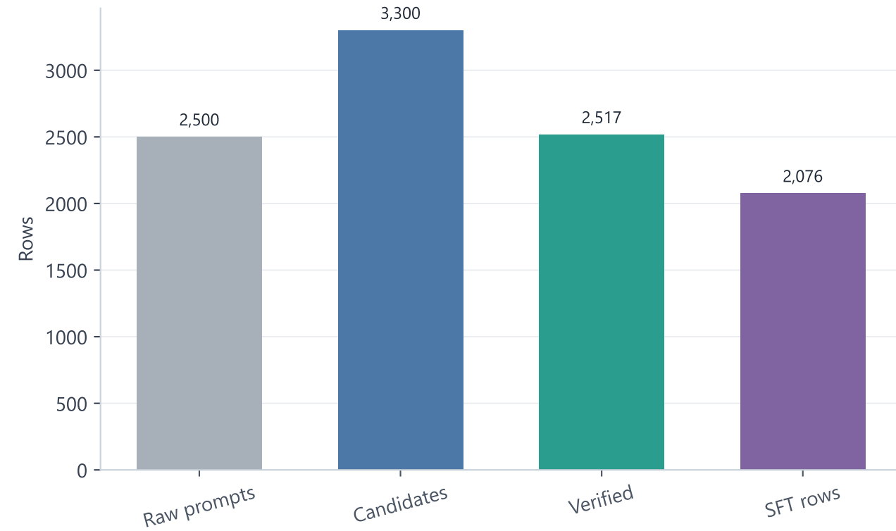
Data-centric construction scale
