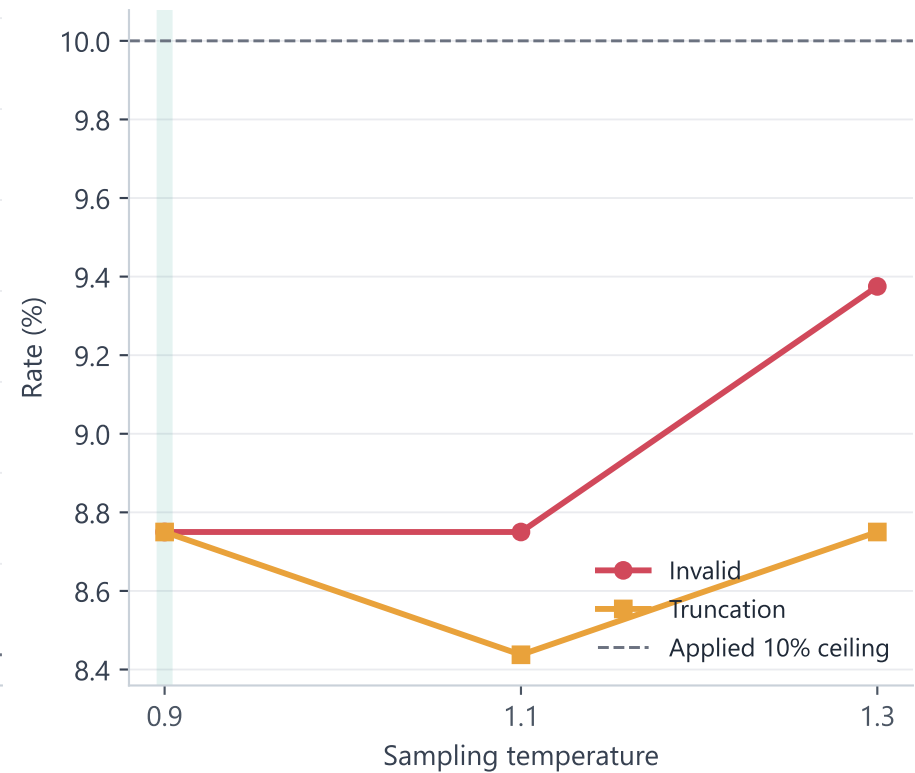
Rollout failure rates
