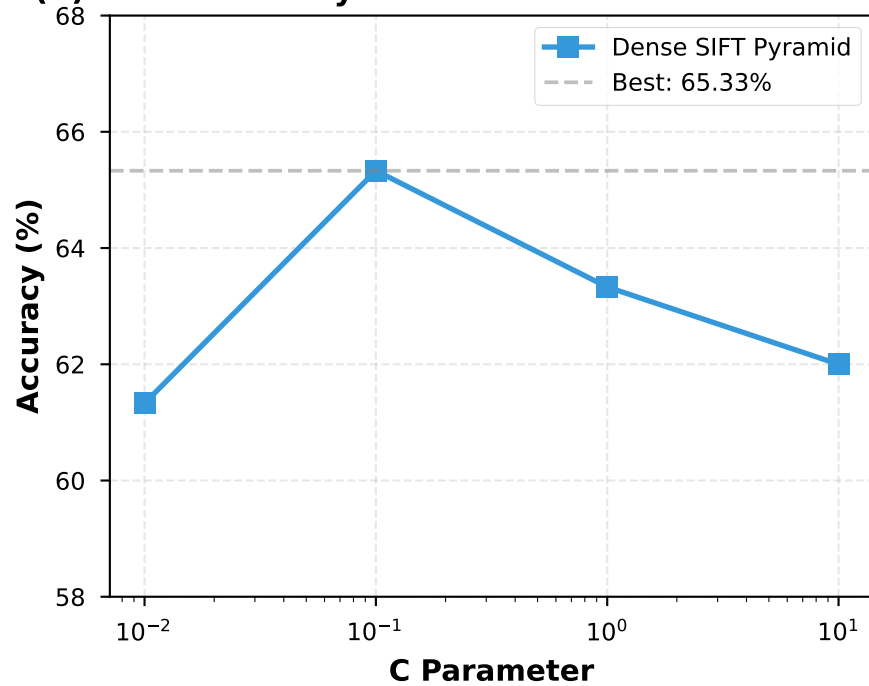
(b) Dense SIFT Pyramid + Chi2 Kernel + LinearSVC
