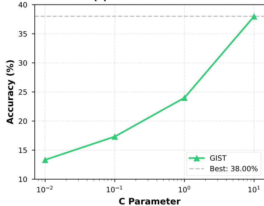
(c) GIST + LinearSVC
