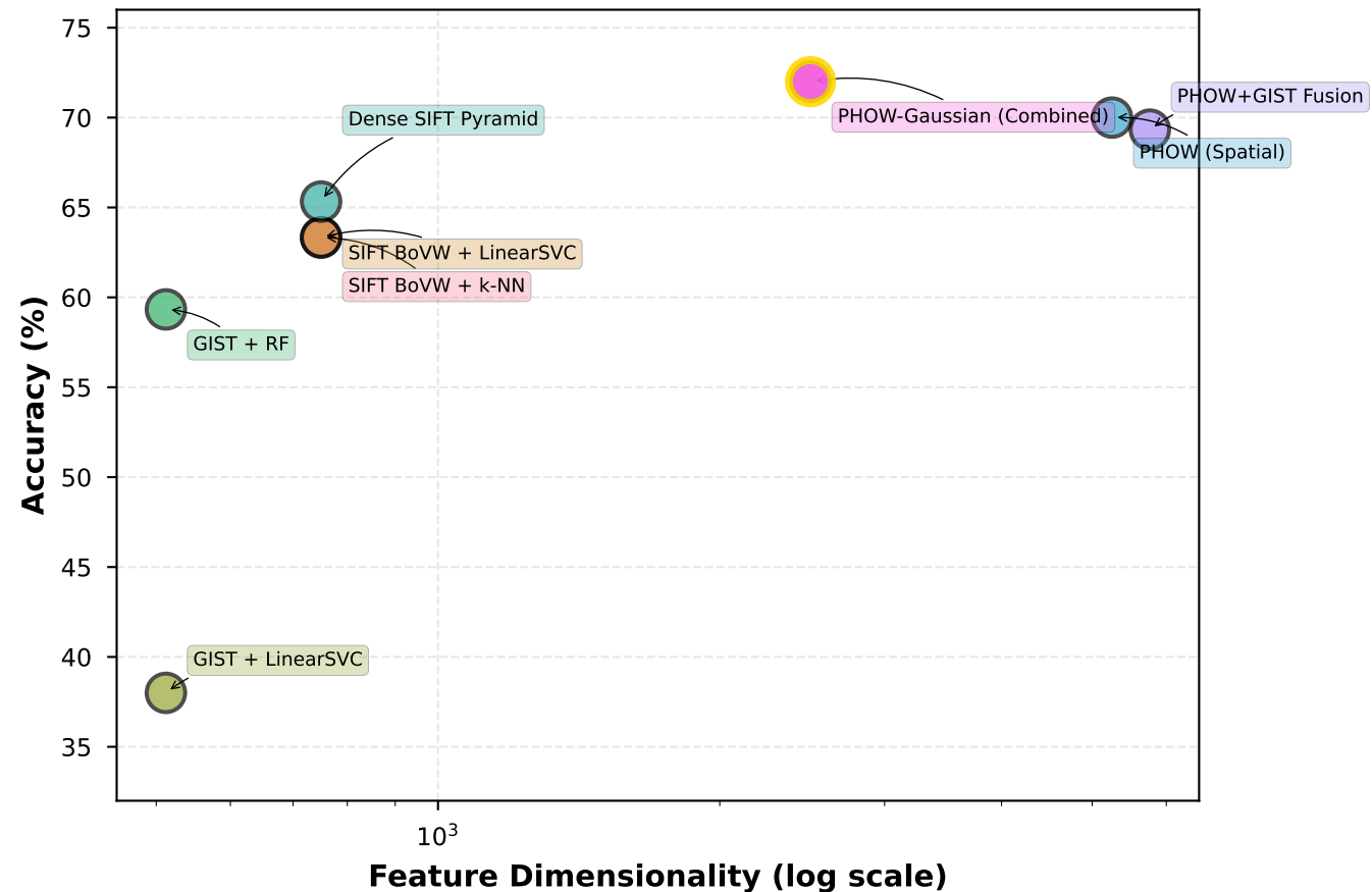
(b) Dimensionality vs Performance Trade-off
