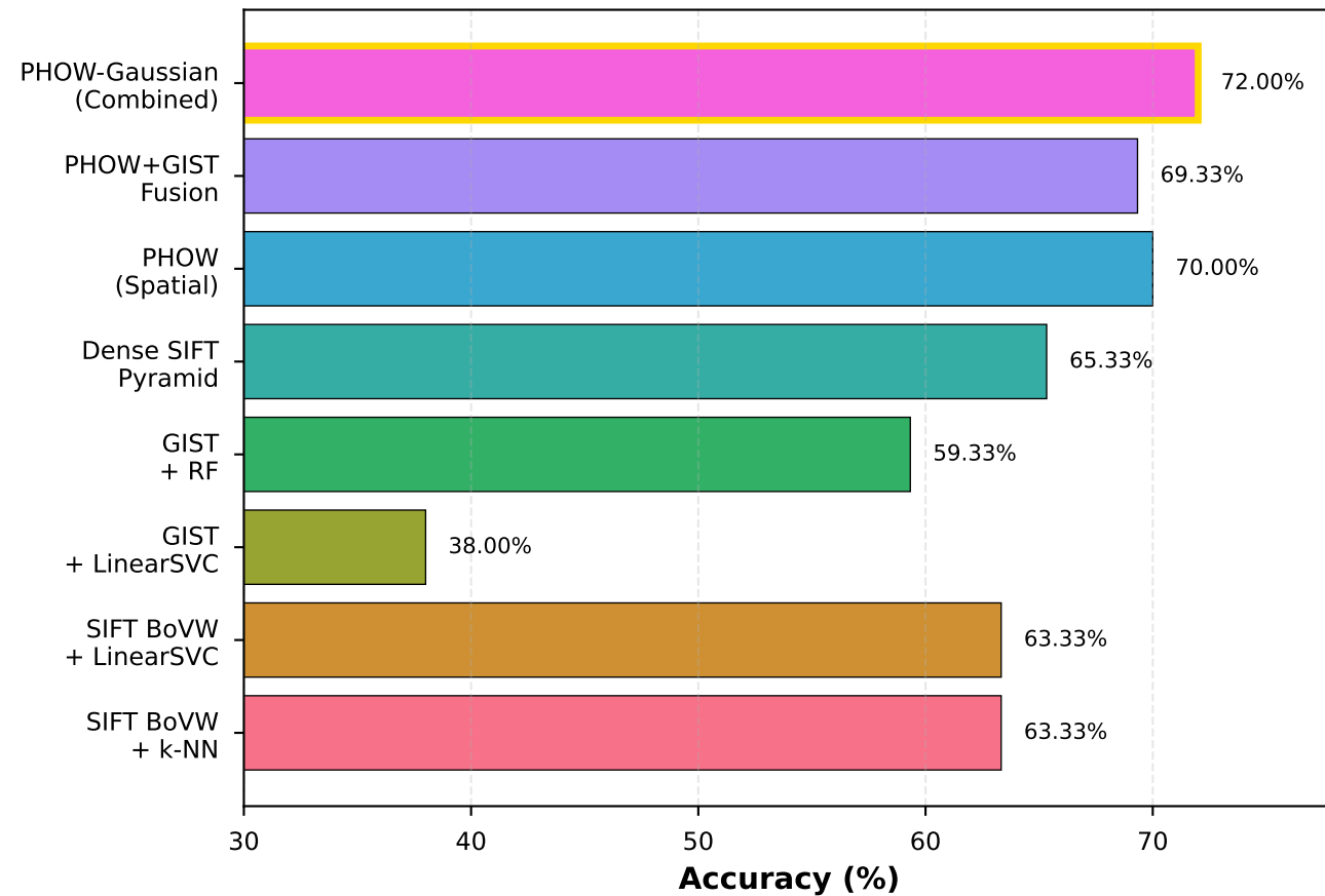
(a) Accuracy Comparison of All Methods
