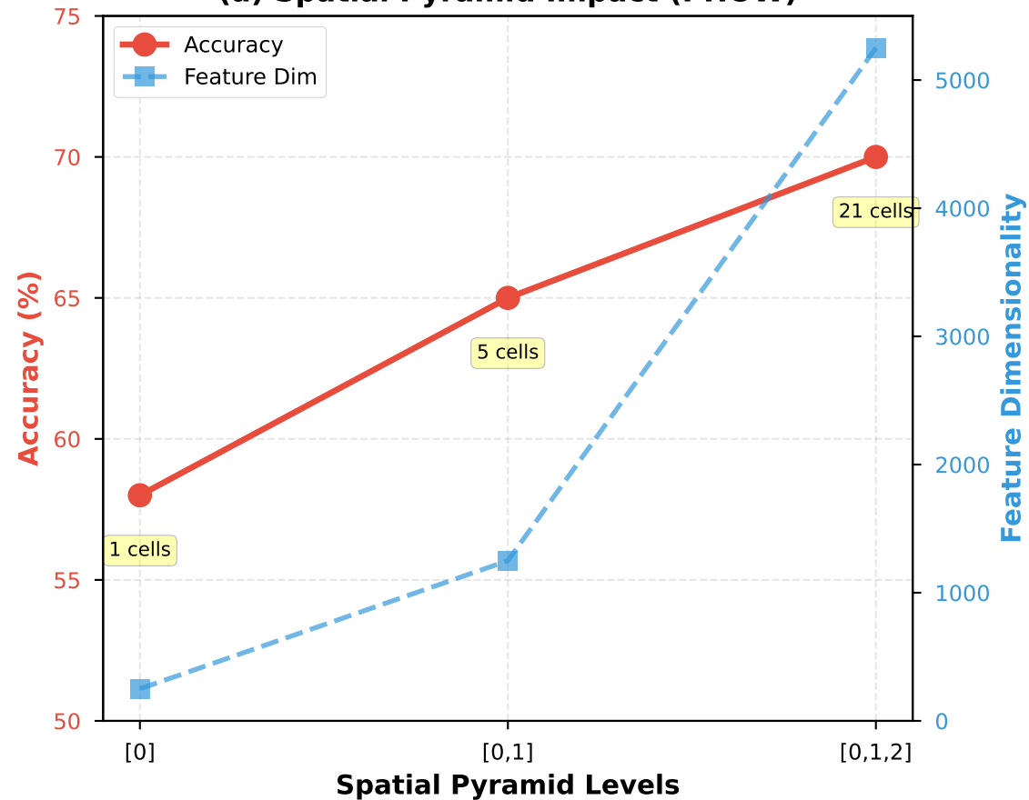
(a) Spatial Pyramid Impact (PHOW)
