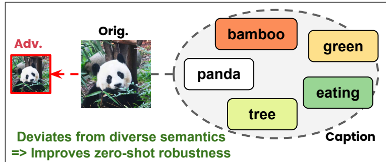
(c) Ours: Supervised w/ Caption
