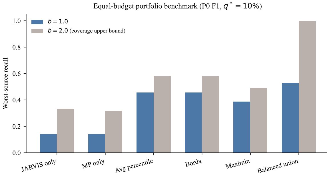
Figure 4: Equal-budget portfolio benchmark on P0 F1 ( q^* = 10\% ). Bars show worst-source recall at budget b = 1.0 (blue) and the coverage upper bound at b = 2.0 (grey). Robust strategies improve worst-source recall relative to single-source selection; the b = 2.0 balanced_union recall of 1.0 is a coverage upper bound by construction.
