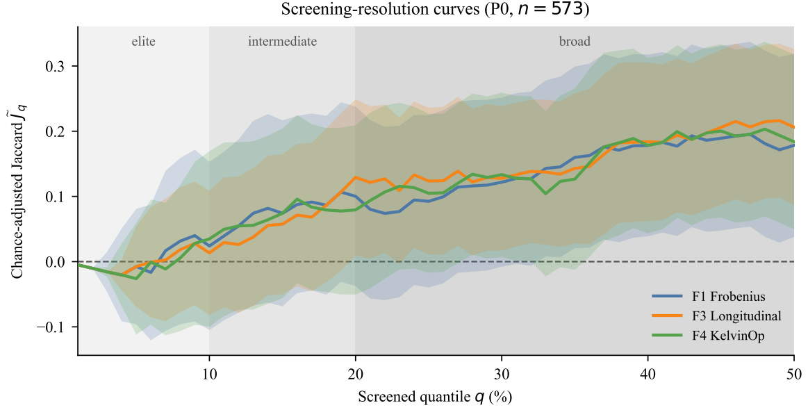
Figure 1: Screening-resolution curves for P0 ( n = 573 ). Solid lines show the chance-adjusted Jaccard overlap \tilde{J}_q for F1 (blue), F3 (orange) and F4 (green); shaded ribbons are simultaneous 95% confidence bands. The horizontal dashed line marks chance-adjusted zero overlap. Background shading distinguishes the elite (1–10%), intermediate (10–20%) and broad (20–50%) bands. Concordance is weak in the elite tail and only becomes positive after substantially broadening the candidate pool.
