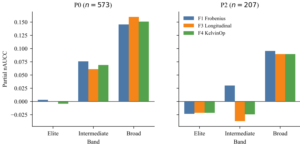
Figure 2: Partial nAUC by band for P0 ( n = 573 ) and P2 ( n = 207 ). Positive values indicate agreement better than chance. For all metrics, concordance is weakest in the elite band and grows only after broadening the candidate pool.
