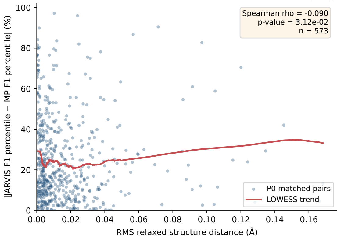
Structure-match distance versus cross-source F1 rank discrepancy
