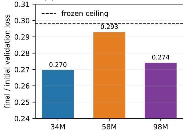
(b) Teacher-forced validation ratio
