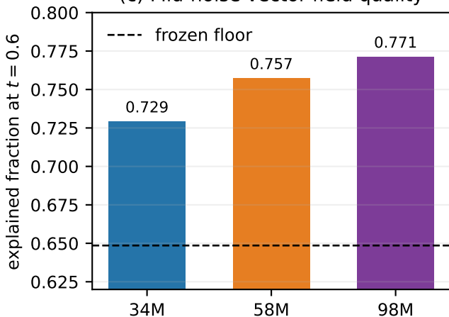
(c) Mid-noise vector-field quality
