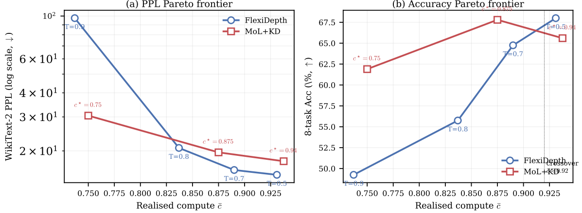
Figure 3: Pareto frontier of FlexiDepth and MoL+KD on Llama-3-8B-Instruct. (a) PPL ( \downarrow , log scale) vs. realised compute \bar{c} . (b) 8-task accuracy ( \uparrow ) vs. realised compute \bar{c} . Points are annotated with each method’s operating-point label. The two curves cross around \bar{c} \approx 0.92 ; above the crossover the methods are within noise, below it MoL+KD strictly dominates on both metrics.
