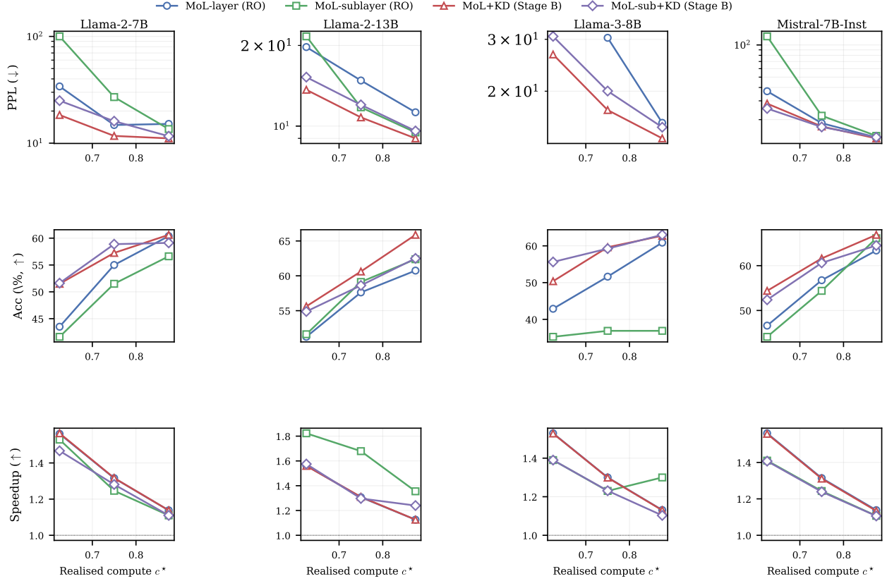
Figure 2: Per-variant Pareto frontier of the four MoL variants across the four per-variant backbones, three metrics. Same data as Table 16: only the four MoL variant curves (layer/sublayer \times router-only/Stage B), plotted for the four backbones with complete per-variant runs (Llama-2-7B, Llama-2-13B, Llama-3-8B, Mistral-7B-Instruct-v0.3). Baseline curves are reproduced in Main Fig. 3. Rows top-to-bottom: WikiText-2 PPL (log, \downarrow ); 8-task Acc (% , \uparrow ); wall-clock decode speedup over the full model ( \uparrow , dotted reference at 1\times ). x : realised compute c^* = L_{\text{eff}}/L . Cells with PPL > 200 are omitted from the PPL row (same omission rule as Table 16).
