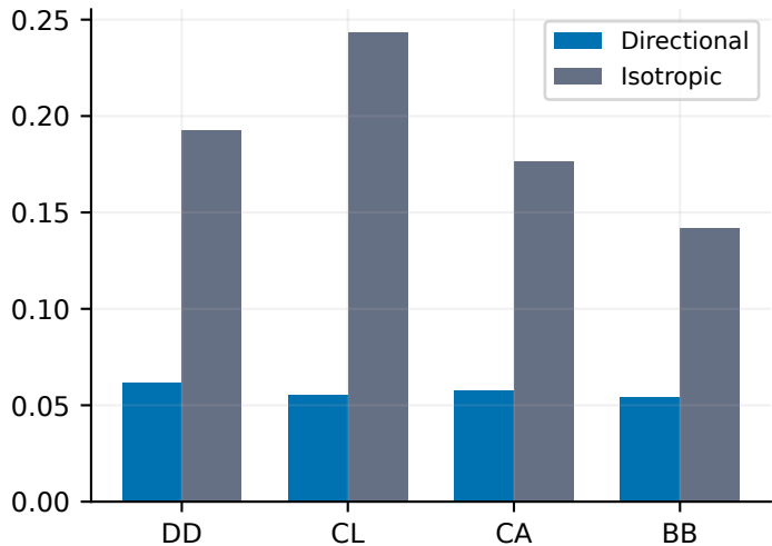
Held-out normalized MAE
