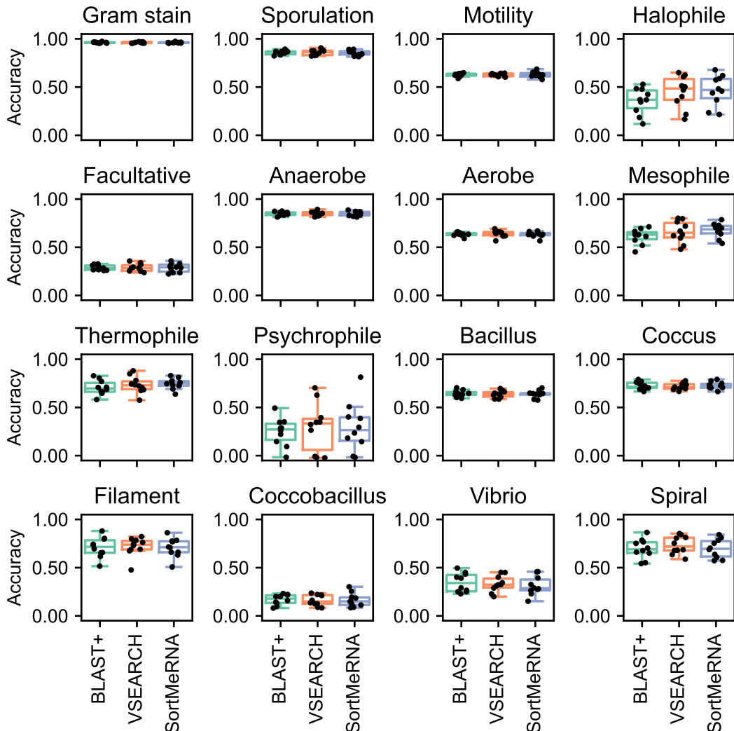
Variation of homology search methods
