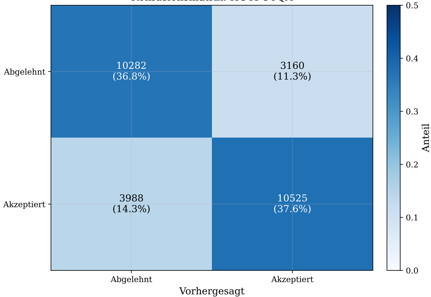
Konfusionsmatrix: HOTPOTQA
