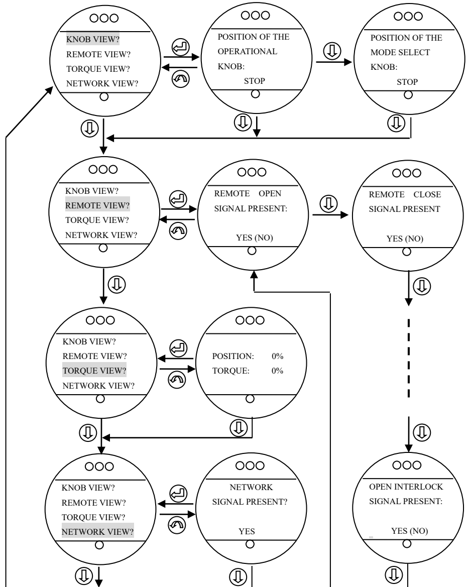
Fig. 4-17 Signal View
