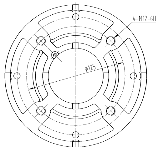
Fig.2-4 RL80-100 Base mounting dimensions
