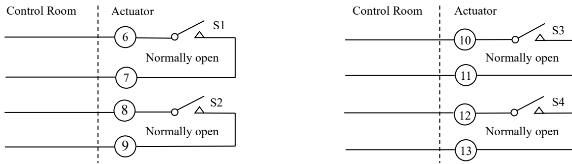
Fig. 9-11 State indication relays
