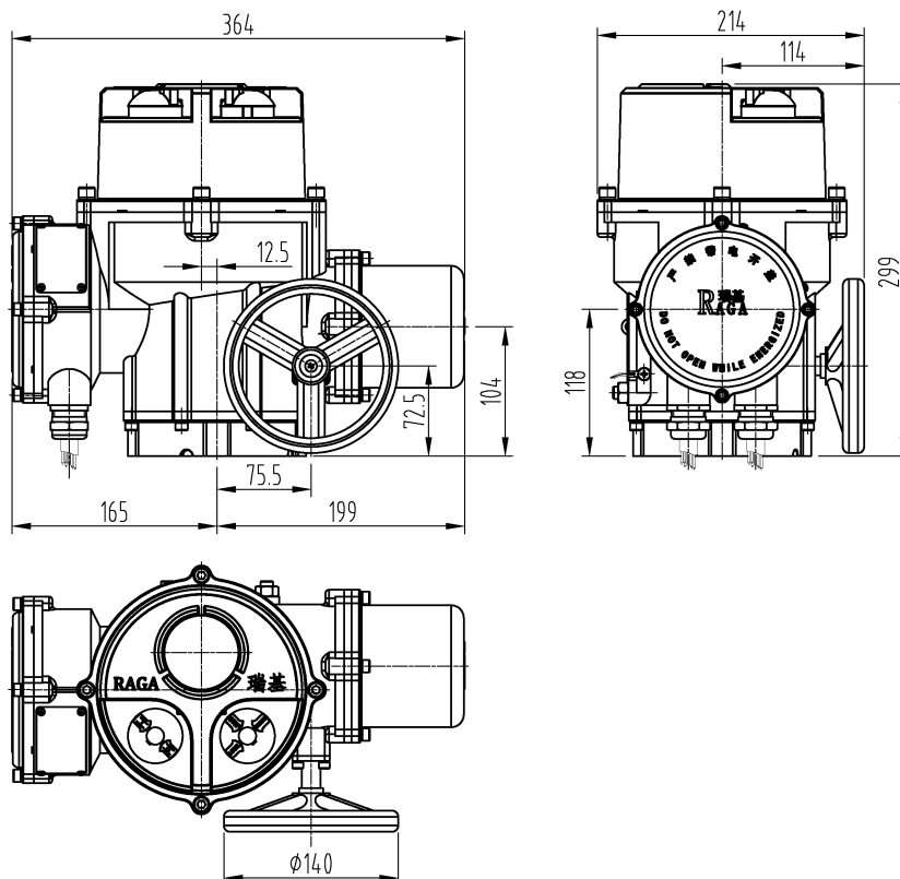
Fig.2-1 Overall dimensions of RL/RLM10-60 Actuator
