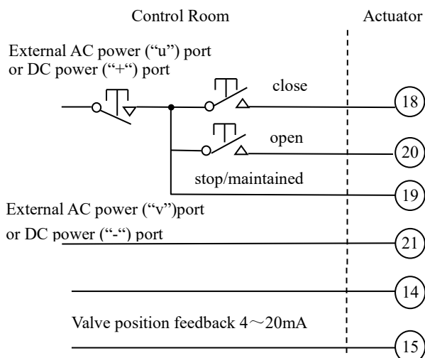
Fig. 9-7 Maintained open/close/stop control
