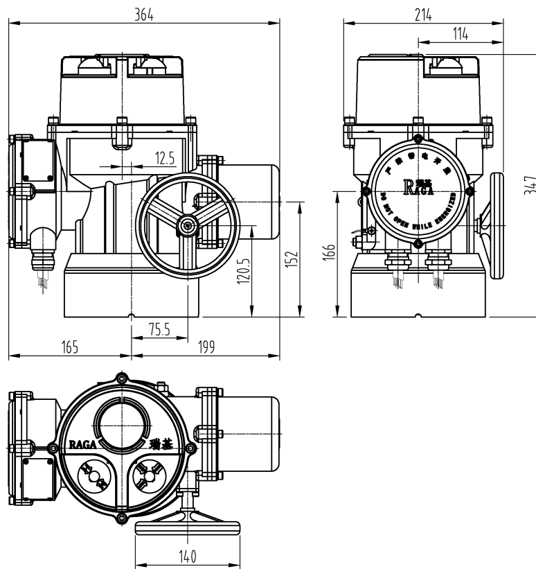
Fig.2-1 Overall dimensions of RL/RLM80-100 Actuator
