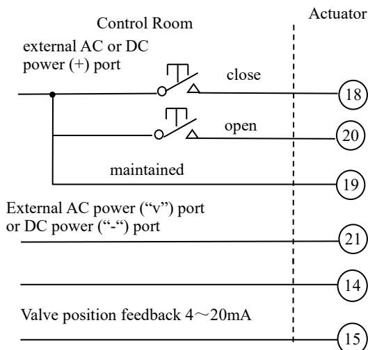
Fig. 9-6 Maintained open / close control, stopping intermediate position is impossible
