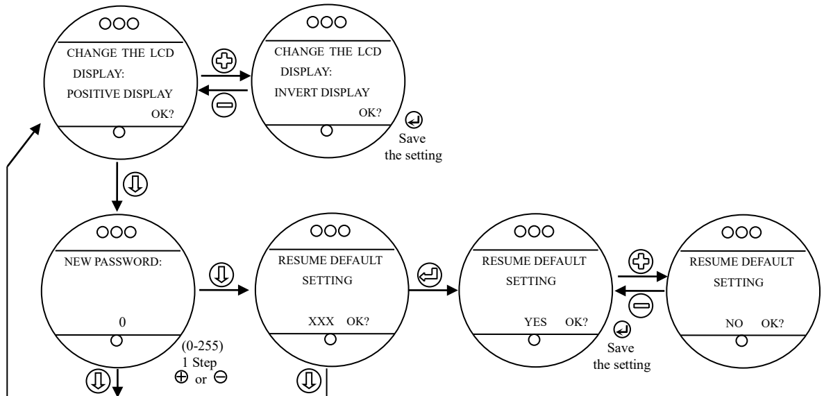
Fig. 4-18 System Setup
