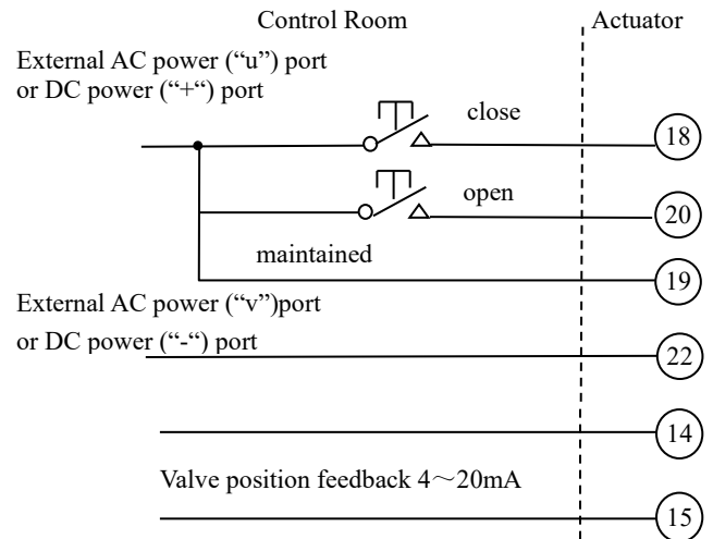
Fig. 9-9 Maintained open / close control, stopping intermediate position is impossible
