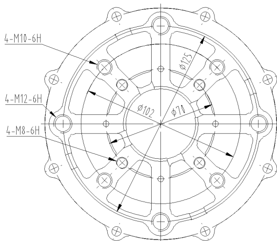
Fig.2-3 RL10-60 Base mounting dimensions
