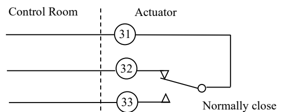
Fig. 9-12 monitor relay wiring diagram
