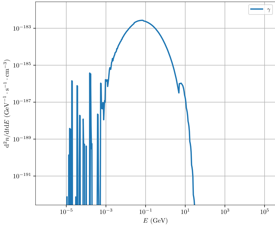
Secondary spectra at t = 2.4 \times 10^{-25} s – test16
