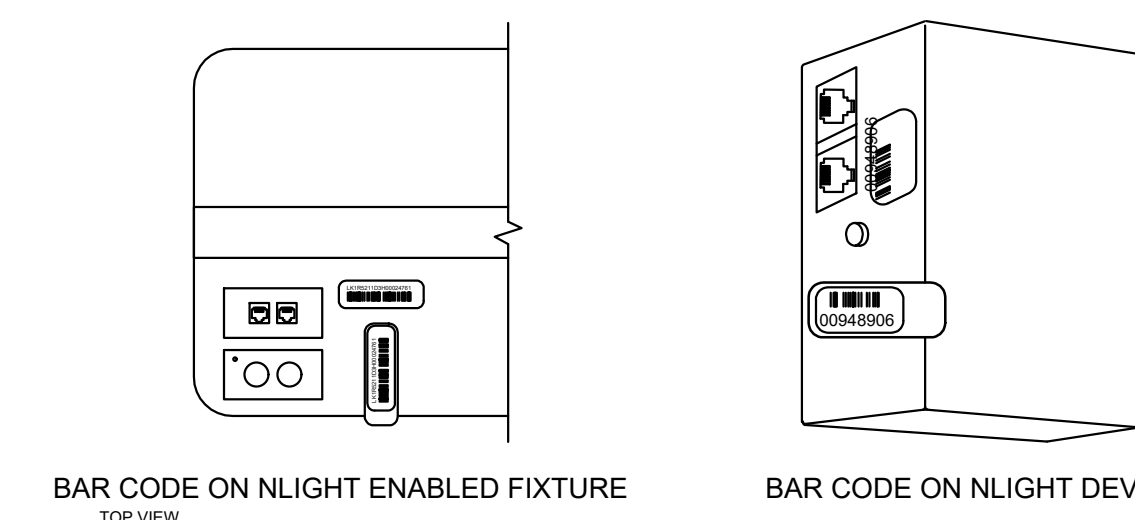
BAR CODE ON NLIGHT ENABLED FIXTURE
