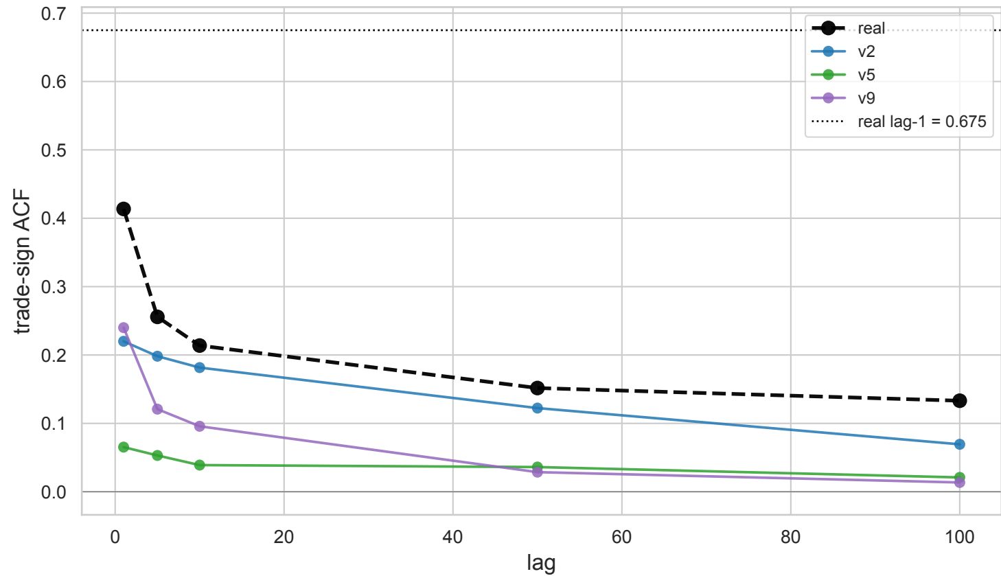
Trade-sign autocorrelation (a key Cont 2001 stylized fact)
