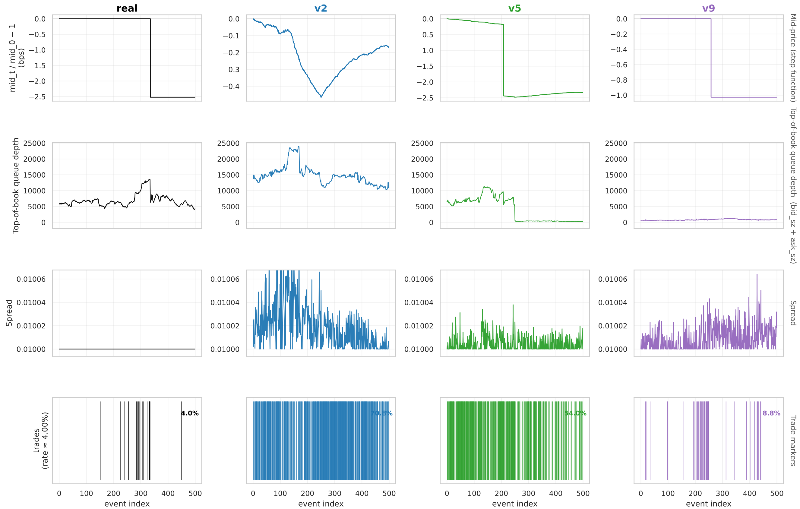
Event-Level Tape Walkthrough — 500 consecutive events from one representative INTC tape per source (mid-price normalized to start; trade rate = fraction of events with trade_sz > 0)
