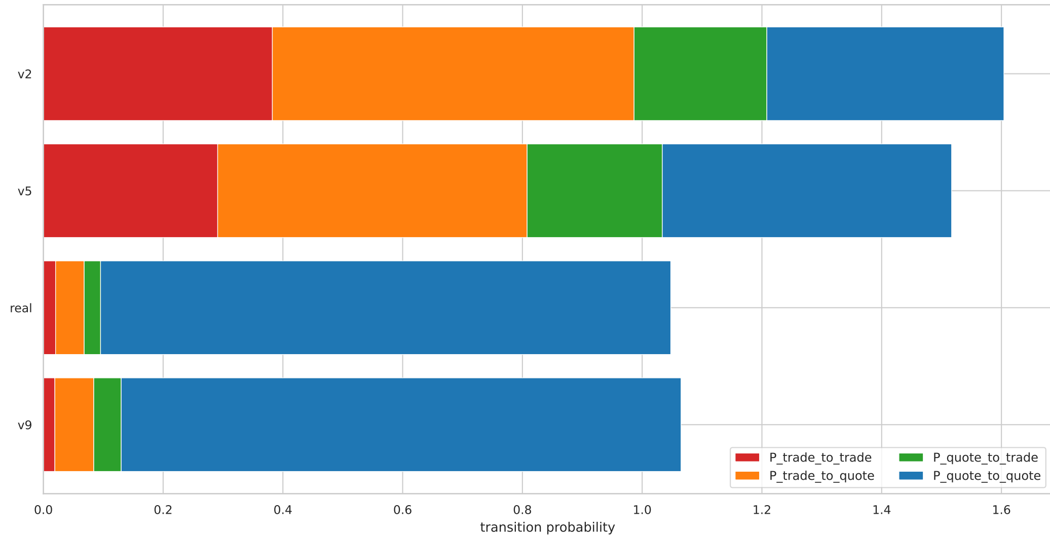
Event-type transition matrix per model (stacked = trade→{trade,quote} + quote→{trade,quote})
