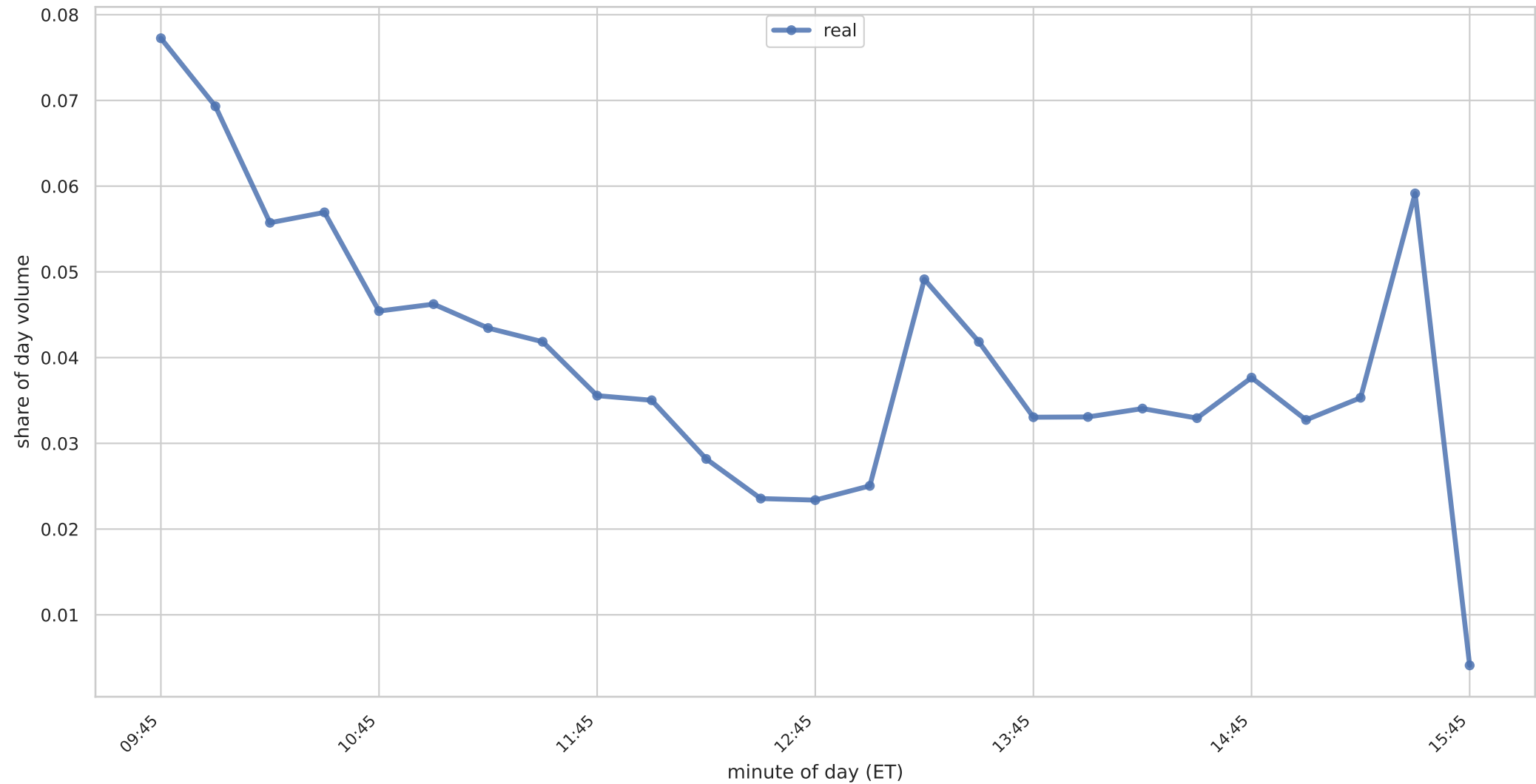
Intraday volume distribution (real should be U-shaped)
