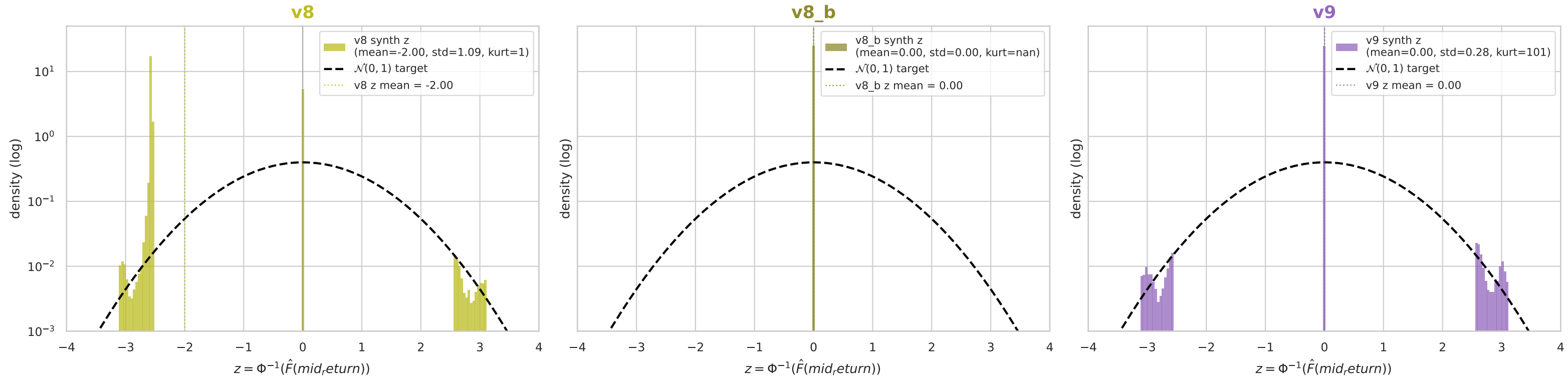
z-Space Collapse and Recovery: copula-transformed mid_{return} for v8 vs v8_b vs v9
