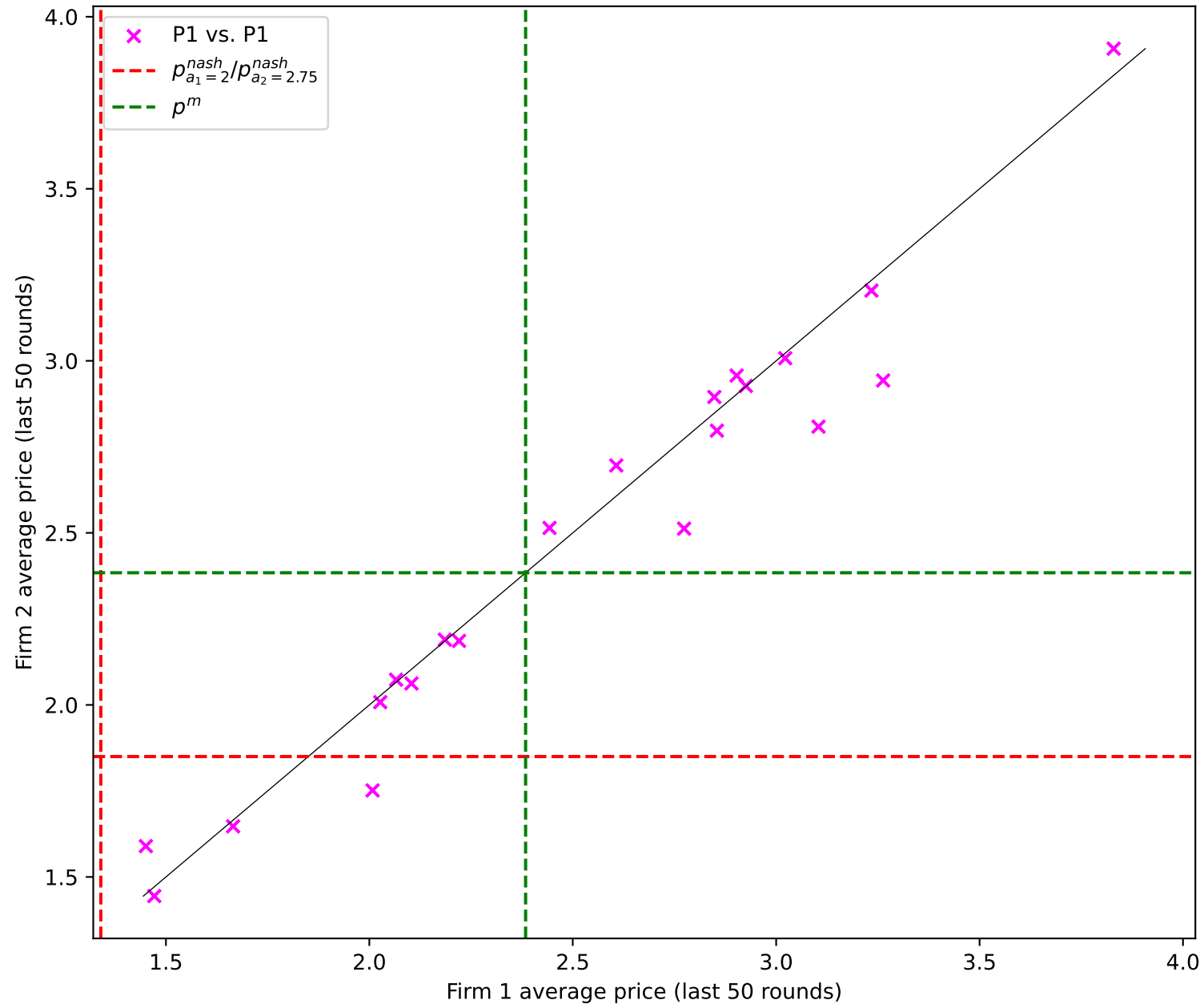
Low-quality ( a_1 = 2 ) vs. High-quality ( a_2 = 2.75 ): Pricing Behavior
