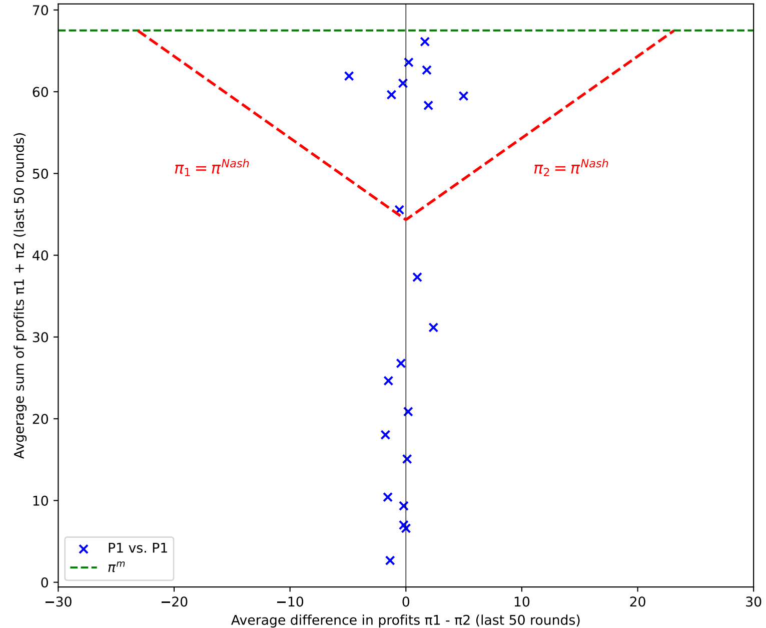
P1 vs P1: Profits Earned
