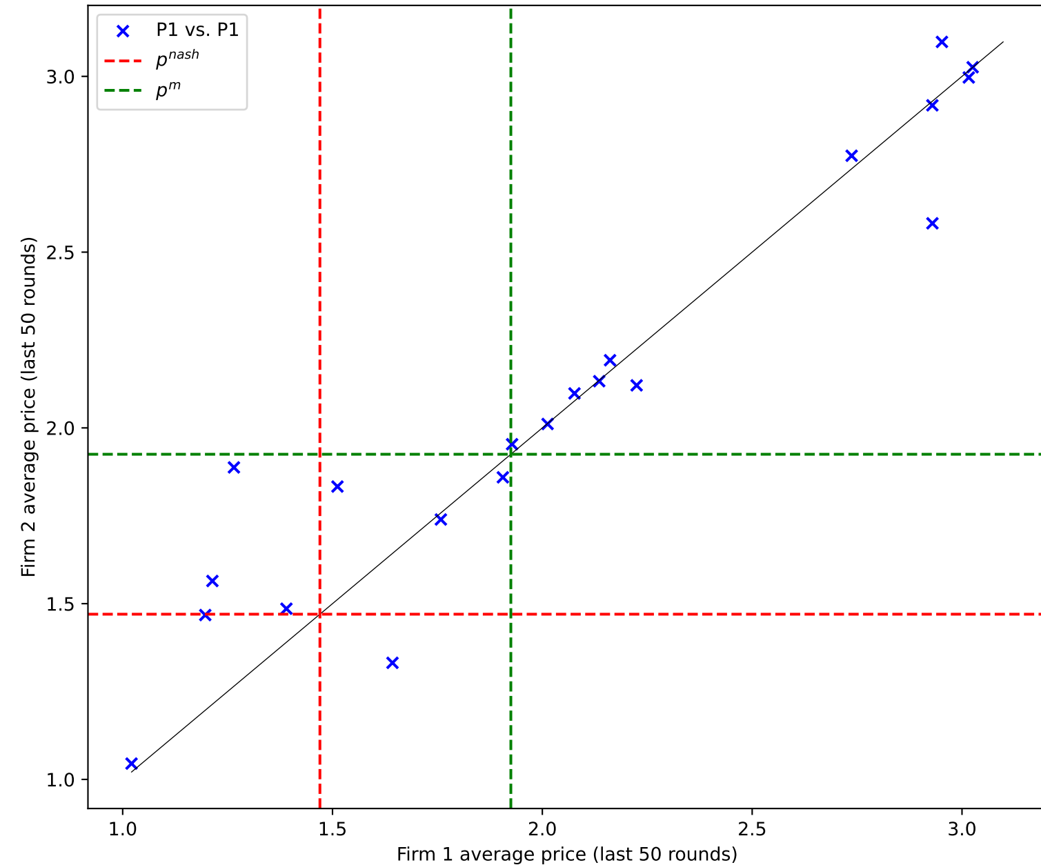
P1 vs P1: Pricing Behavior
